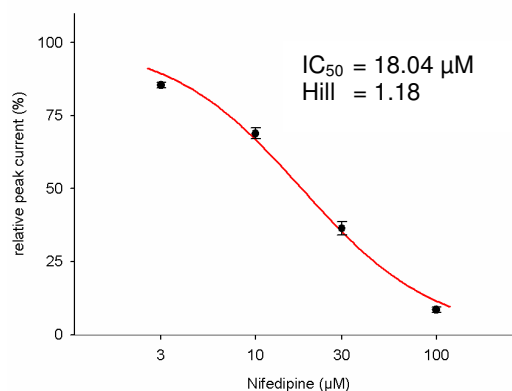
Fig. 3.1.2.2: K V 1.2 peak current inhibition curve of Nifedipine. The inhibition curve was best fitted with an IC 50 value of 18.04 μM, Hill Coefficient: 1.18 (n=4)
