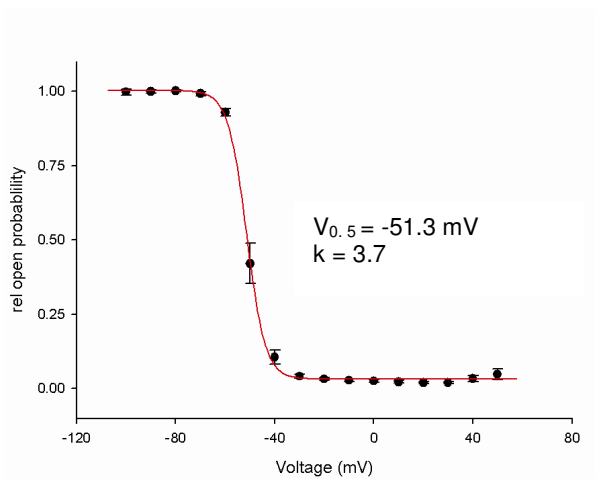
Fig. 2.1.4.1: Inactivation plot of Kv1.4 tail currents fitted to Boltzmann function with V_{0.5} = -51.3 \text{ mV} , k = 3.7 ( n = 6 cells).
