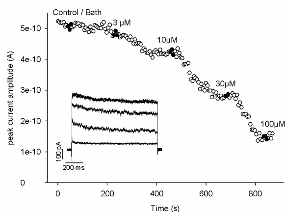
Fig. 3.1.1.1: Long time course of a CHO K v 1.1 cell. Peak current amplitude was reduced by increasing concentrations of Nifedipine.
