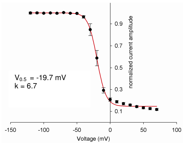
Fig. 2.1.3.1: Inactivation plot of Kv1.3 tail currents fitted to Boltzmann function with V_{0.5} = -19.7 \text{ mV} , k = 6.7 ( n = 4 cells).
