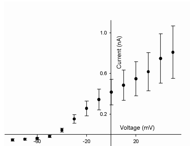
Fig. 2.1.1.2: IV curve of K V 1.1 activation currents. Voltages between -120 and +70 mV were applied ( n = 11 ).
