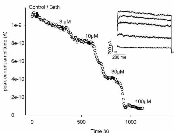
Fig. 3.1.2.1: Long time course of a CHO K V 1.2 cell. Peak current amplitude was reduced by increasing concentrations of Nifedipine.
