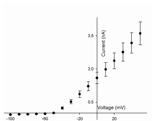
Fig. 2.1.4.2: IV curve of Kv1.4 activation currents. Voltages between -100 and +50 \text{ mV} were applied.
