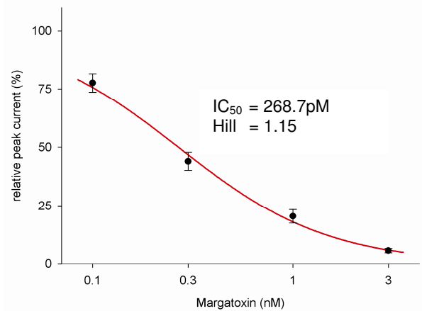
Fig. 3.1.3.2: K v 1.3 peak current inhibition curve of Margatoxin. The inhibition curve was best fitted with an IC 50 value of 268.7 pM, Hill Coefficient: 1.15 (n=4)
