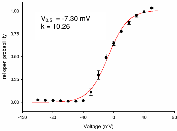
Fig. 2.1.5.1: Activation plot of Kv1.5 tail currents fitted to Boltzmann function with V_{0.5} = -7.30 mV, k = 10.26 ( n = 4 cells).
