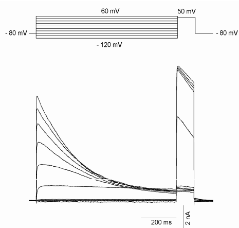
Fig. 1.1.3: Representative K v 1.3 outward currents recorded upon depolarization of the CHO membrane from a holding potential of -80 mV to voltages between -120 mV and +60 mV in 20 mV increments (800 ms). Voltage pulses to 50 mV (100 ms) elicited K v 1.3 tail currents.
