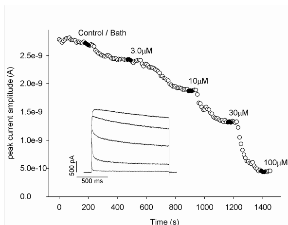
Fig. 3.1.5.1: Long time course of a CHO K v 1.5 cell. Peak current amplitude was reduced by increasing concentrations of Nifedipine.
