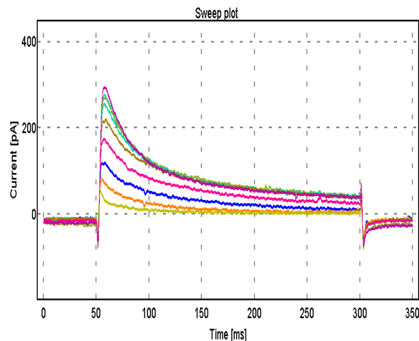
Fig. 3.1.4.3: Long time course of a CHO K v 1.4 cell. Peak current amplitude was reduced by increasing concentrations of Quinidine.
