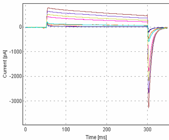
Fig. 3.1.3.3: Long time course of a CHO K v 1.3 cell. Peak current amplitude was reduced by increasing concentrations of Margatoxin.
