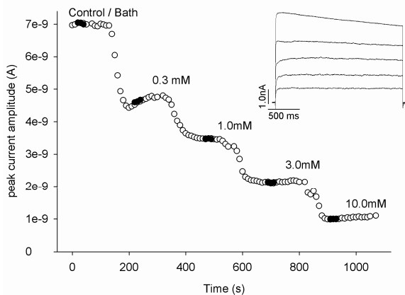
Fig. 3.1.6.1: Long time course of a CHO K v 1.6 cell. Peak current amplitude was reduced by increasing concentrations of 4-AP.
