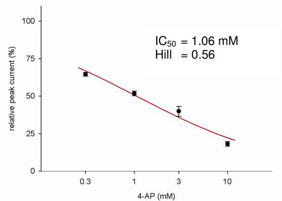
Fig. 3.1.6.2: K v 1.6 peak current inhibition curve of 4-AP. The inhibition curve was best fitted with an IC 50 value of 1.06 mM, Hill Coefficient: 0.56 (n=5)
