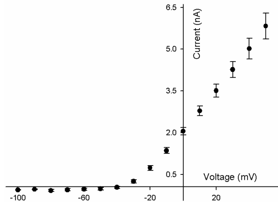
Fig. 2.1.5.2: IV curve of Kv1.5 activation currents. Voltages between -100 and +50 mV were applied.
