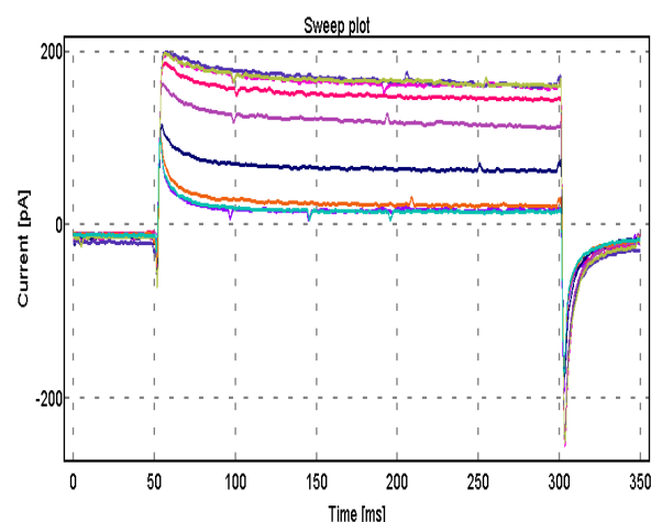
Fig. 3.1.1.3: Long time course of a CHO K v 1.1 cell. Peak current amplitude was reduced by increasing concentrations of Hongotoxin.
