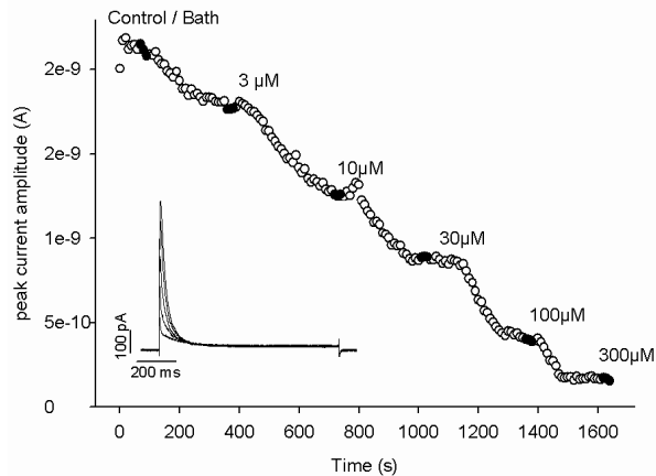
Fig. 3.1.4.1: Long time course of a CHO K v 1.4 cell. Peak current amplitude was reduced by increasing concentrations of Quinidine.
