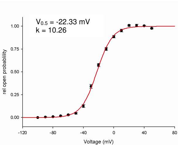
Fig. 2.1.6.1: Activation plot of Kv1.6 tail currents fitted to Boltzmann function with V_{0.5} = -22.33 mV, k = 10.26 ( n = 9 cells).
