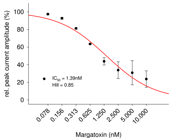
Fig. 3.1.3.4: K v 1.3 peak current inhibition curve of Margatoxin. The inhibition curve was best fitted with an IC 50 value of 1.39 nM, Hill Coefficient: 0.85 for the instantaneous current amplitude.
