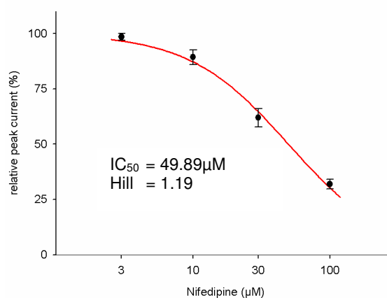
Fig. 3.1.1.2: K v 1.1 peak current inhibition curve of Nifedipine. The inhibition curve was best fitted with an IC 50 value of 49.89 μM, Hill Coefficient: 1.19 (n=3)
