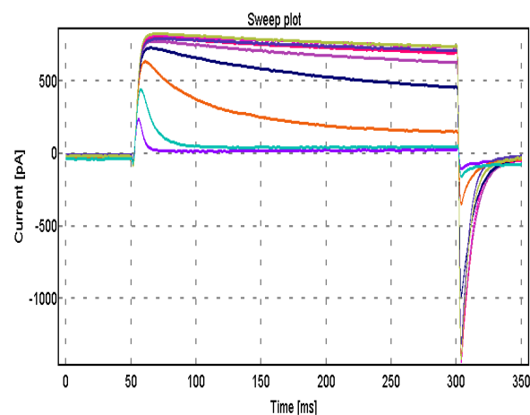
Fig. 3.1.5.3: Long time course of a CHO K v 1.5 cell. Peak current amplitude was reduced by increasing concentrations of S9947.
