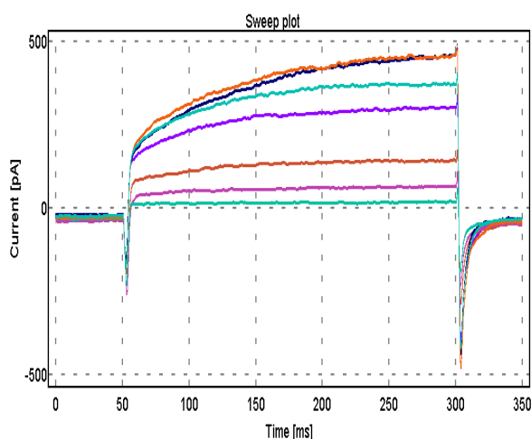
Fig. 3.1.2.3: Long time course of a CHO K V 1.2 cell. Peak current amplitude was reduced by increasing concentrations of Hongotoxin.
