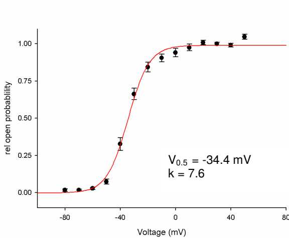
Fig. 2.1.1.1: Activation plot of K V 1.1 tail currents fitted to Boltzmann function with V_{0.5} = -34.4 mV, k = 7.6 ( n = 6 cells).
