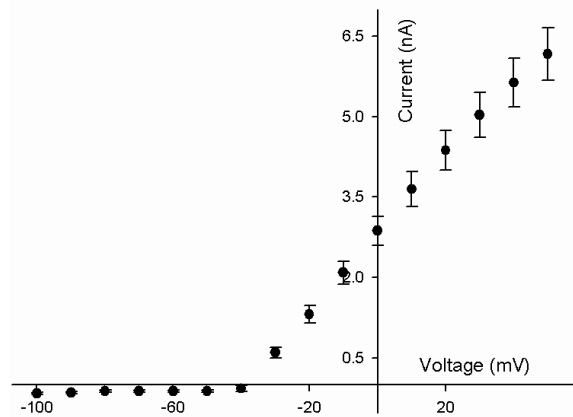
Fig. 2.1.6.2: IV curve of Kv1.6 activation currents. Voltages between -100 and +50 mV were applied.
