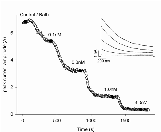
Fig. 3.1.3.1: Long time course of a CHO K v 1.3 cell. Peak current amplitude was reduced by increasing concentrations of Margatoxin.
