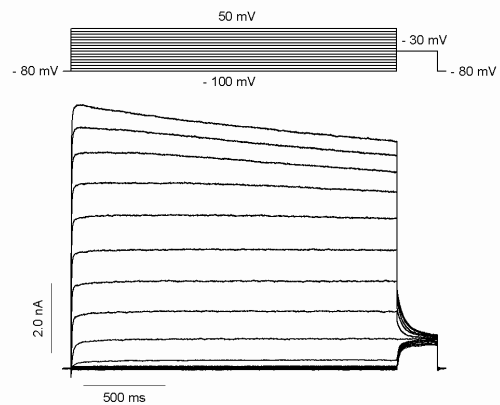
Fig. 1.1.6: Representative K v 1.6 outward currents recorded upon depolarization of the CHO membrane from a holding potential of -80 mV to voltages between -100 mV and +50 mV in 10 mV increments (2000 ms). Voltage pulses to -30 mV (250 ms) elicited K v 1.6 tail currents.
