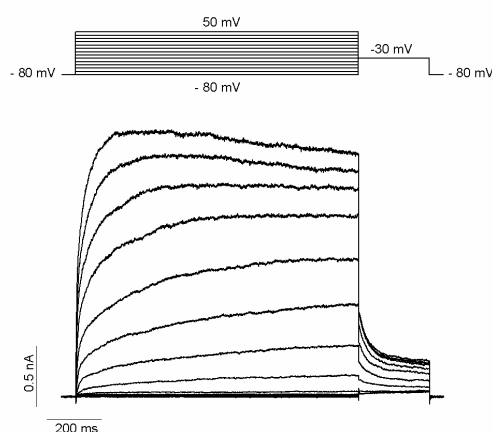
Fig. 1.1.2: Representative K V 1.2 outward currents recorded upon depolarization of the CHO membrane from a holding potential of -80 mV to voltages between -80 mV and +50 mV in 10 mV increments (1000 ms). Voltage pulses to -30 mV (300 ms) elicited K V 1.2 tail currents.
