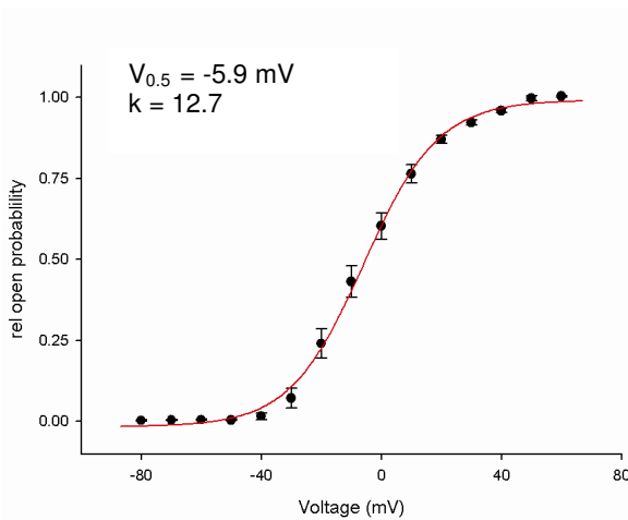
Fig. 2.1.2.1: Activation plot of K V 1.2 tail currents fitted to Boltzmann function with V_{0.5} = -5.9 mV, k = 12.4 ( n = 6 cells).
