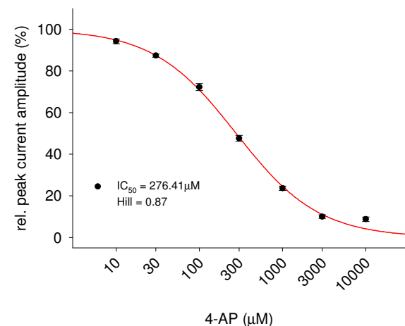
Fig. 3.1.6.4: K v 1.6 peak current inhibition curve of 4-AP. The inhibition curve was best fitted with an IC 50 value of 276.41 μM, Hill Coefficient: 0.87 for the instantaneous current amplitude.
