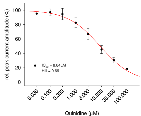
Fig. 3.1.4.4: K v 1.4 peak current inhibition curve of Quinidine. The inhibition curve was best fitted with an IC 50 value of 8.84 μM, Hill Coefficient: 0.69 for the instantaneous current amplitude.
