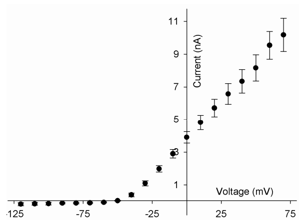
Fig. 2.1.3.2: IV curve of Kv1.3 activation currents. Voltages between -120 and +70 \text{ mV} were applied.
