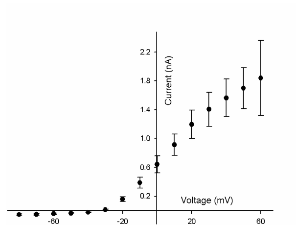
Fig. 2.1.2.2: IV curve of K V 1.2 activation currents. Voltages between -80 and +60 mV were applied.
